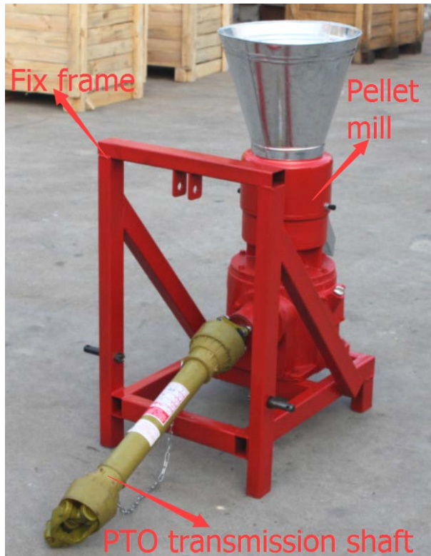
PTO pellet mill structure
